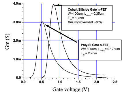
Fig. 3 Transconductance comparison between \text{CoSi}_2 and poly gated devices
