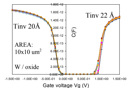
Fig. 6 Inversion CV curves for W/oxide p-FETs and n-FETs
