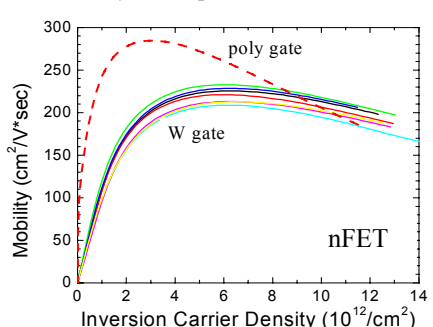
Fig. 12 W and poly gate n-FET mobility
