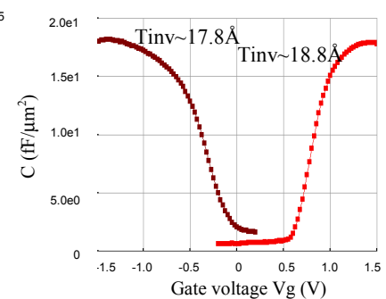
Fig. 9 W/oxynitride C vs. V_g curves
