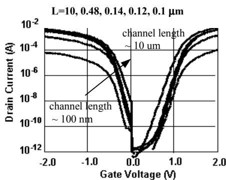
Fig. 7 W/oxide I_d vs. V_g curves
