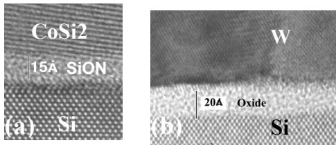
Fig. 1. TEM cross-sections of (a) \text{CoSi}_2 gate on 15\text{\AA} Si-oxynitride and (b) W/ 20\text{\AA} \text{SiO}_2 gate stack
