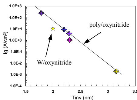
Fig. 10 I_g vs. T_{\text{inv}} comparing poly / W gated devices
