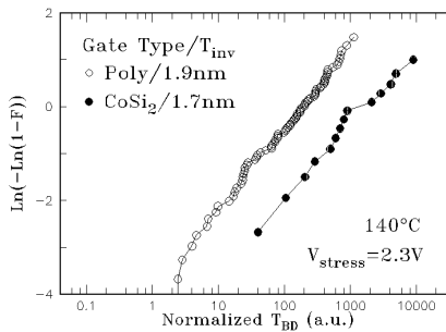
Fig. 5 Better time to breakdown characteristic for \text{CoSi}_2 compared to poly gated devices
