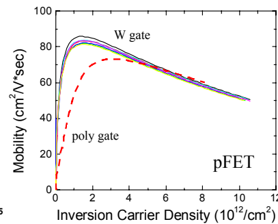
Fig. 11 W and poly gate p-FET mobility
